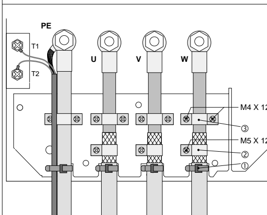
FIG 4-17 Proposal for motor connection with 822X
