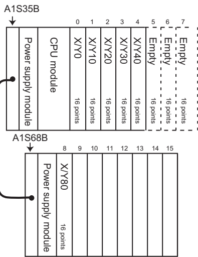
(1) Setting the start XY address of each slot
