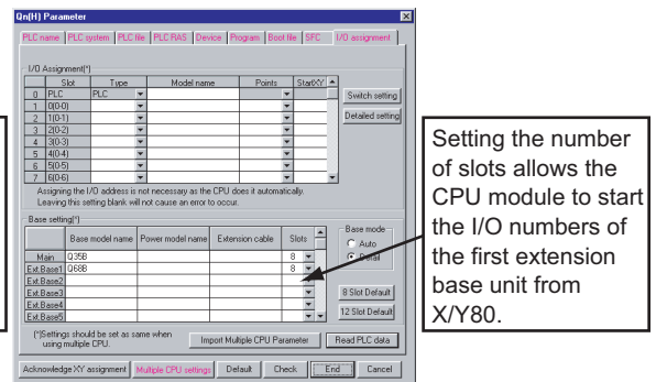
(2) Setting the number of slots to "8"
