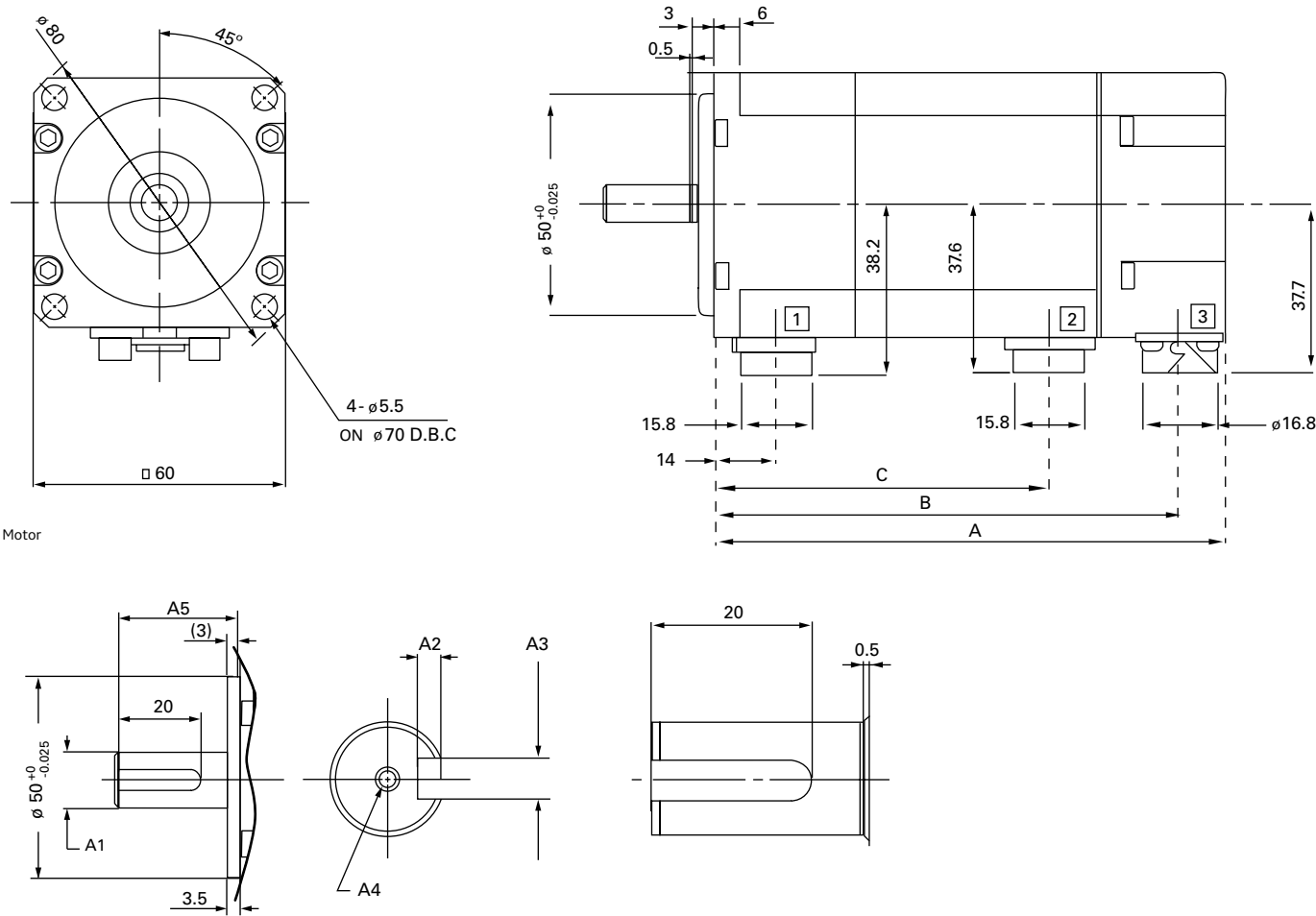
Shaft detail
