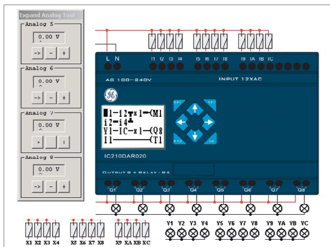
Ladder Logic
